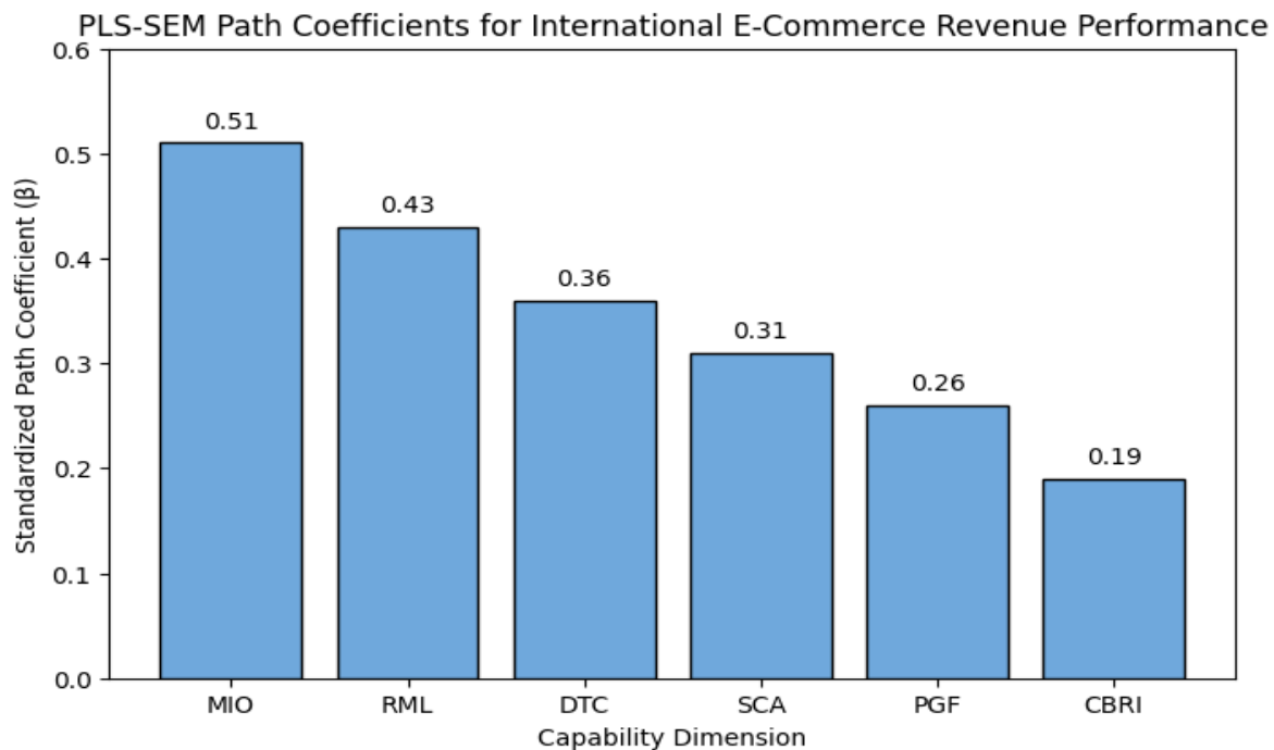
Figure 2: PLS-SEM Path Coefficients for International E-Commerce Revenue Performance
