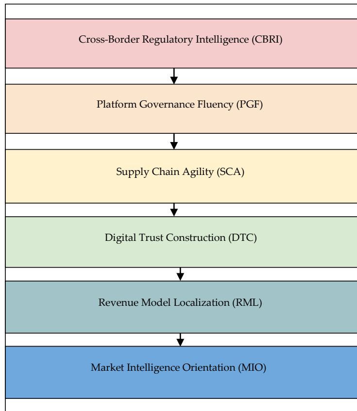
Figure 1: E-Commerce Market Penetration Ladder (EMPL) Hierarchy
