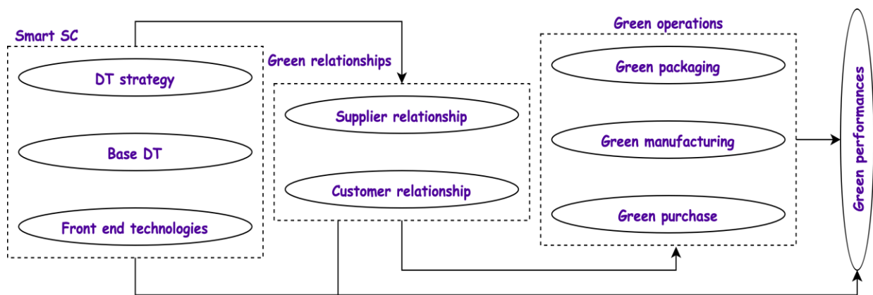
Figure 3: SSCM Architecture
