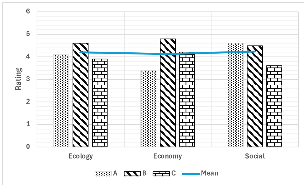
Figure 4: SSCM Analysis
